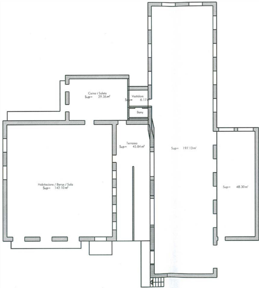
PLANTAC QUARTA
